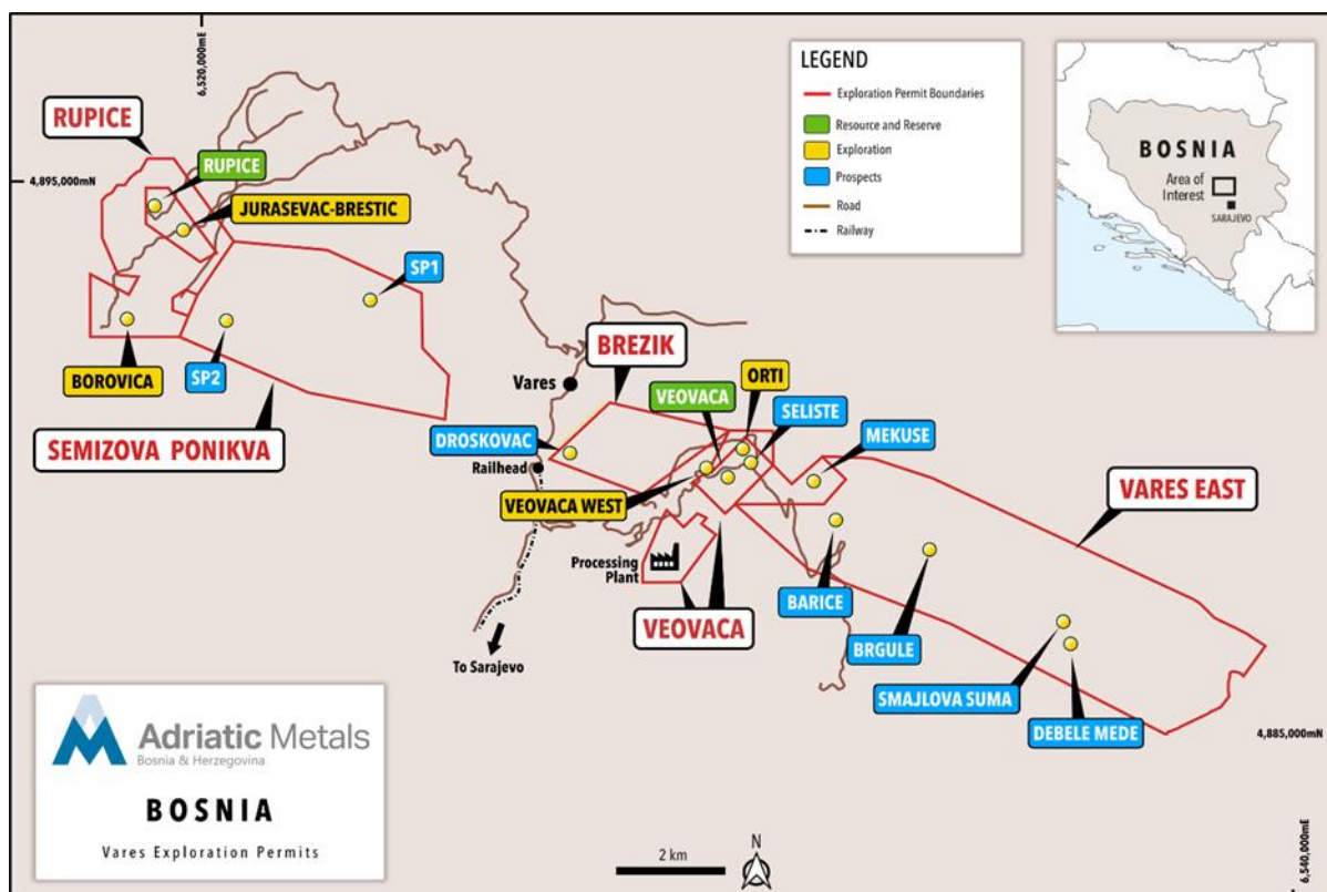
Figure 1. Map showing the location of Vares Project
